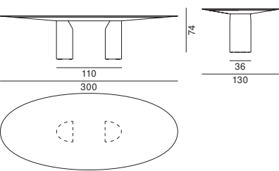
Oval table L300
