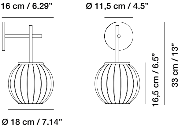
Difusor A / Diffuser A
