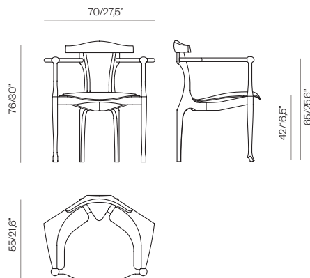
GAULINO EASYCHAIR
